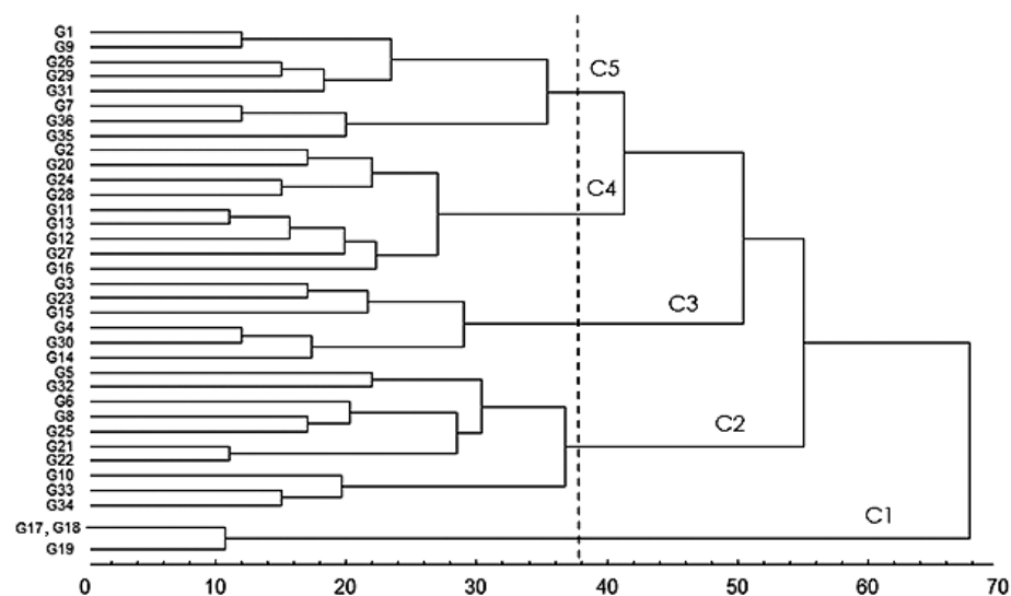
Figure 2. Cluster analysis of Aegilops geniculata accessions from Algeria based on gliadin polymorphism using Ward's method
